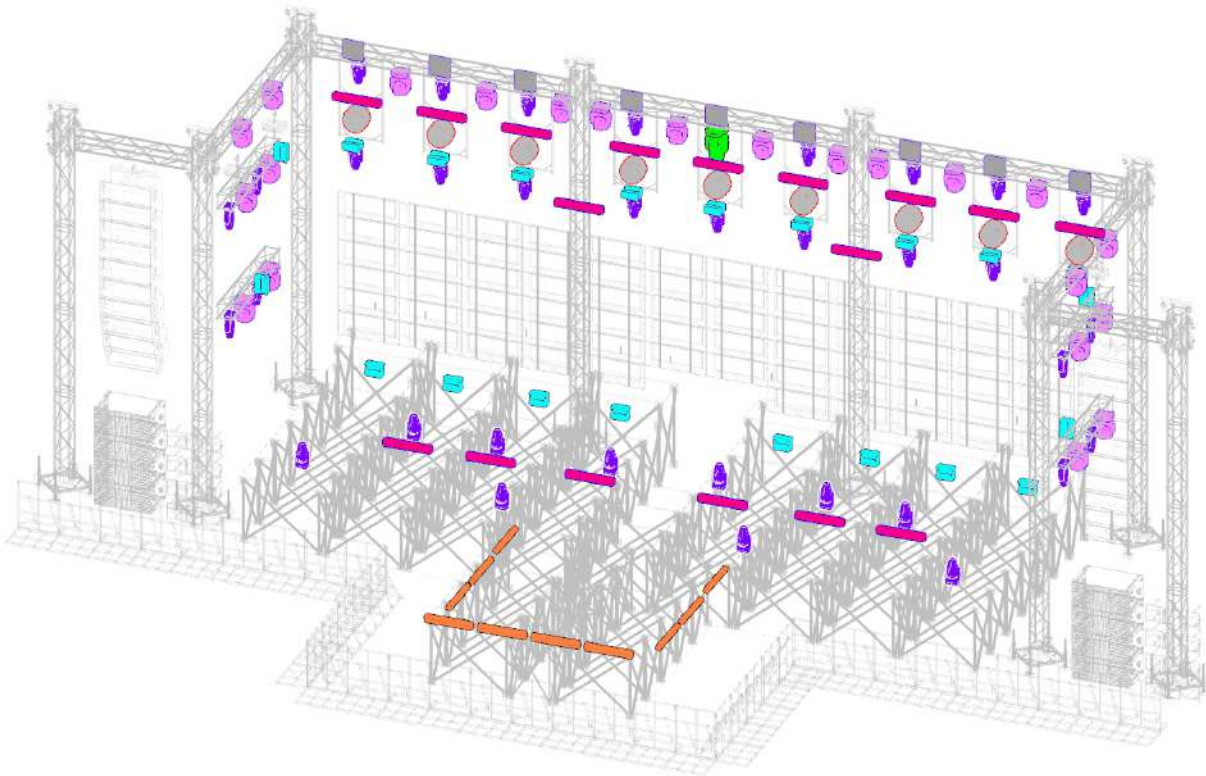
L.P :: Isometric View
