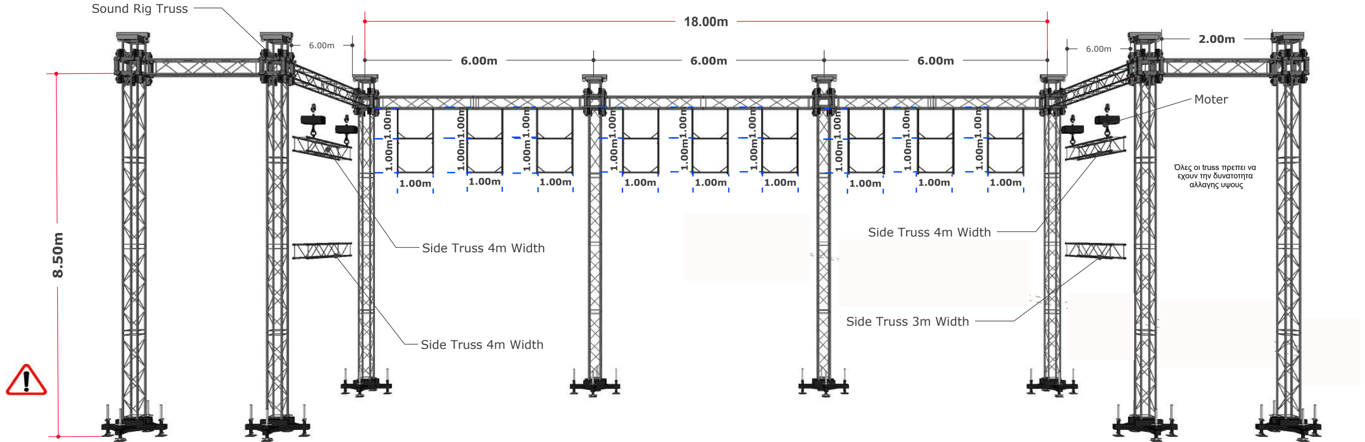
TRUSS :: Front View
