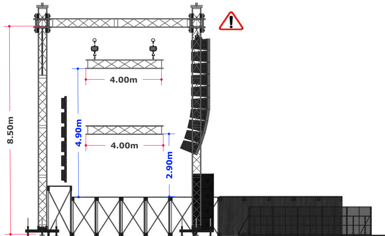
TRUSS :: Left View
